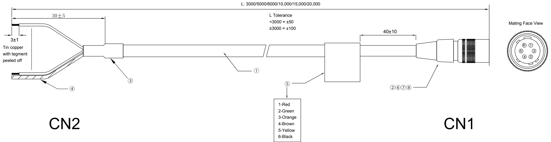
Wiring Diagram
