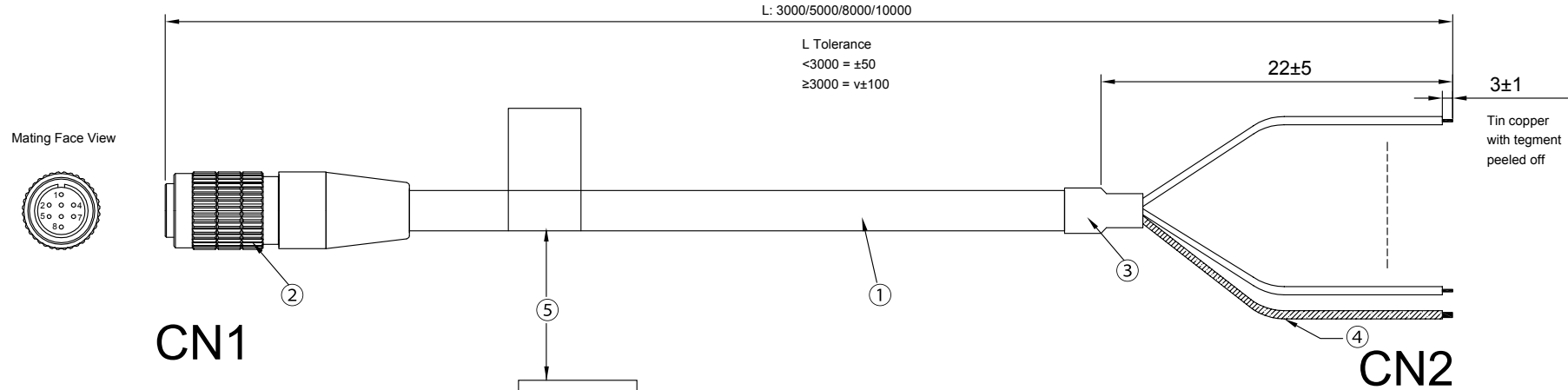
Wiring Diagram
