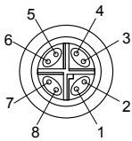
Mating Face View
